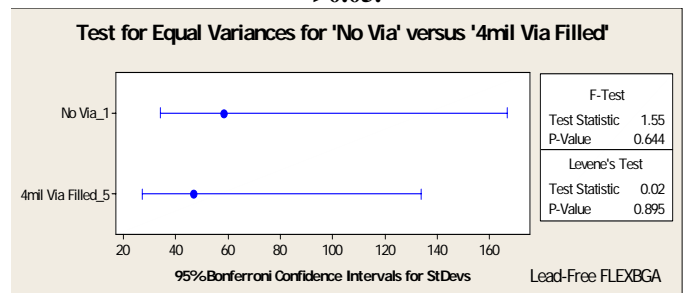
Figure 31 - Results for 'Test for equal variance' in 0.8mm 280 I/O BGA with lead-free alloy. Again, P-values are >0.05.
